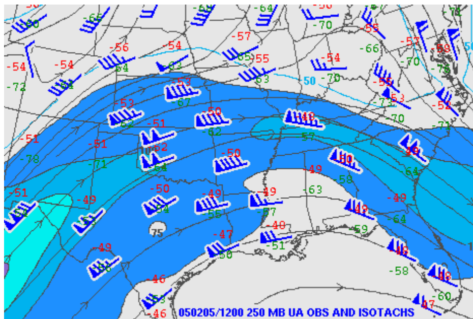
Figure 5. A 250hPa analysis is shown, valid at 1200 UTC, 5 February 2005. Contours and shading are the same as in Figure 3. (Source: NOAA/SPC)
