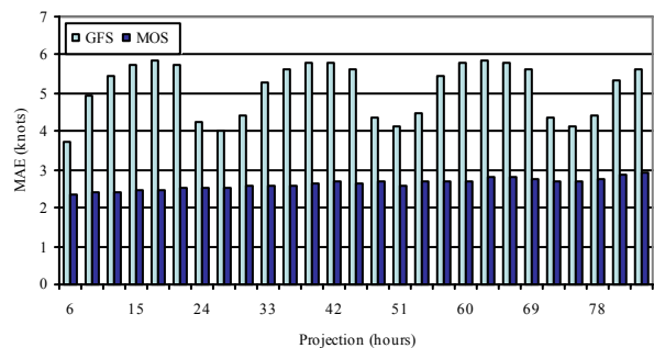
Figure 1. Comparison of overall mean absolute errors (MAE) in wind speed, MOS versus GFS forecasts, dry season, 0000 UTC, for 15 stations.
