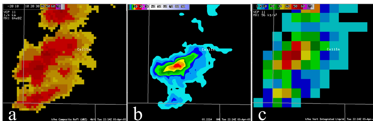
Figure 6. (a) KFWs Composite Reflectivity showing 35 dBz and higher values at 2214 UTC on 05 April 2005; (b) FED imagery at 2214 UTC; (c) KFWs VIL imagery at 2214 UTC. The FED imagery effectively highlighted the most significant convection in southwest Collin County.
