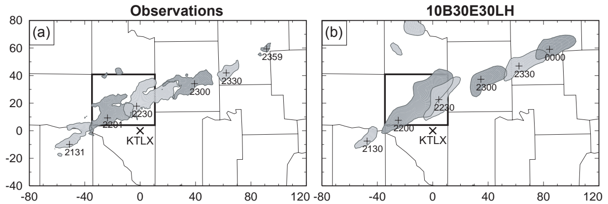
Fig. 3. As in Fig. 2, but for (a) 2130, 8 May to 0000, 9 May 2003, at 30 minute intervals, and (b) the corresponding predicted fields from experiment 10B30E30LH. Regions with reflectivity exceeding 45 dBZ are shown. The locations of the maximum reflectivity of the OKC storm are marked by + signs together with the corresponding times. The domain shown represents the portion of the 3-km grid between 210 and 410 km in east-west direction and from 260 to 380 km in north-south direction.
