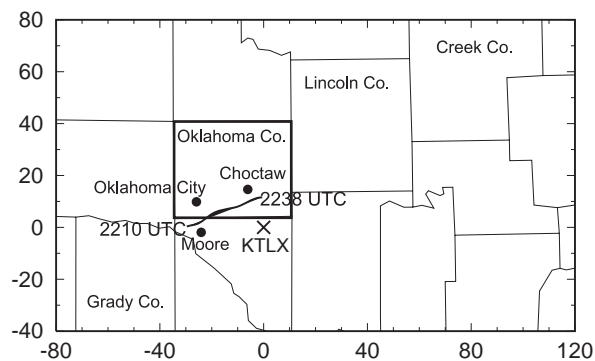
Fig. 1. Map of counties and cities related to the 8 May 2003 OKC tornadic thunderstorm. The dark line segment starting at 2210 northwest of Moore and ending at 2238 south Choctaw marks the rough path of the OKC tornado. The x and y distances are in kilometer and are relative to the KTLX radar marked by x in the figure. The Oklahoma County is highlighted.
