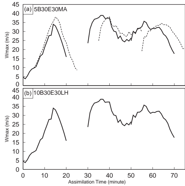
Fig. 7. The maximum vertical velocities for the first 20 minutes of forecasts starting from analyses at 0 (2030), 30 (2100), and 50 (2120) minutes into the assimilation cycles (solid lines) and from the analyses following the above analyses (dash lines), for experiments 5B30E30MA (a) and 10B30E30LH (b).
