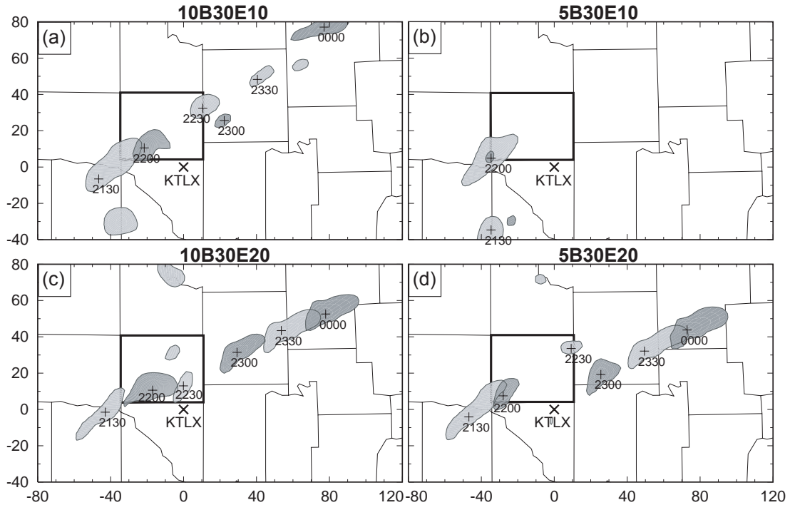
Fig. 11. As Fig. 3b, but for experiments 10B30E10 (a), 10B30E20 (c), 5B30E10 (b), and 5B30E20 (d).
