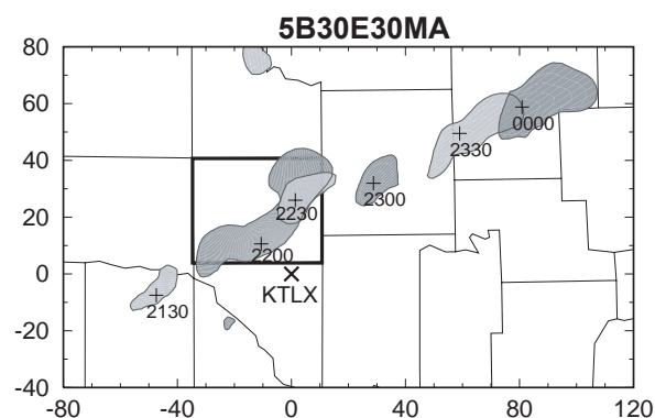
Fig. 5. As Fig. 3b, but for experiment 5B30E30MA.
