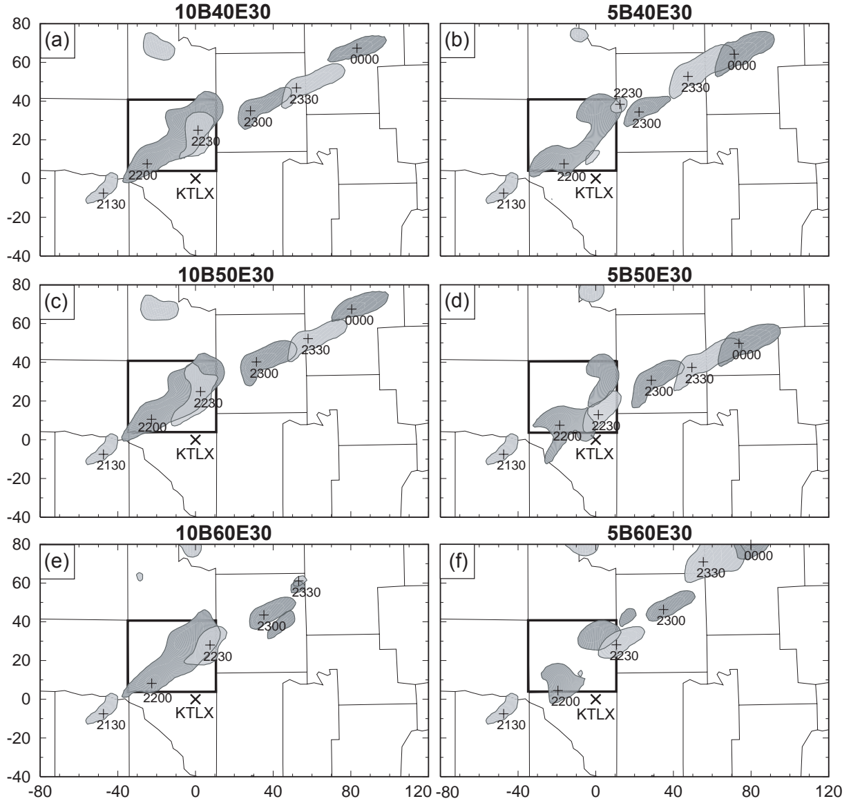
Fig. 12. As Fig. 3b, but for experiments 10B40E30 (a), 10B50E30 (c), 10B60E30 (e), 5B40E30 (b), 5B50E30 (d), and 5B60E30 (f).
