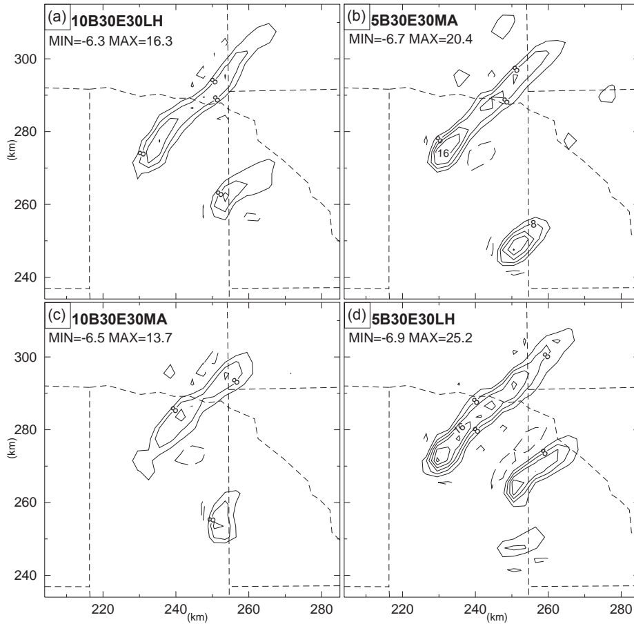
Fig. 10. The vertical velocity fields at 7 km MSL at the end of assimilation in experiments 10B30E30LH (a), 5B30E30MA (b), 10B30E30MA (c), and 5B30E30LH (d). The domain shown represents the portion of 3-km grid between 205 and 285 km in east-west direction and from 235 to 315 km in north-south direction. The contour interval is 4 \text{ ms}^{-1} .
