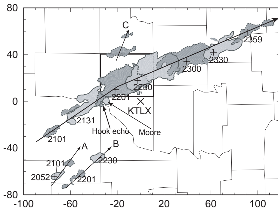
Fig. 2. Regions of radar echoes exceeding 35 dBZ as observed by KTLX radar at the 1.45° elevation. The echoes are at 30-minute intervals from 2101 to 2359, of 8 May 2003. The grayscales of the echoes at two consecutive times are different, so are their outlines. The locations of the maximum reflectivity are marked by + signs, together with the corresponding times. The x and y coordinates are in kilometers and have their origin at the KTLX radar site that is marked by x. The arrow lines are the trajectories of the OKC storm and the storms A, B, and C. Also, the look echo at 2201 and Moore are pointed by arrows. The Oklahoma County is highlighted.
