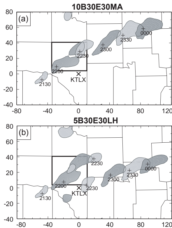
Fig. 8. Same as Fig. 3b, but for experiments 10B30E30MA (a) and 5B30E30LH (b).
