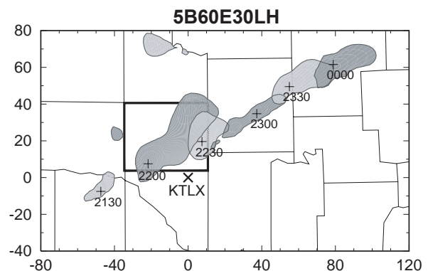
Fig. 13. As Fig. 3b, but for experiment 5B60E30LH.
