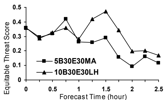
Fig. 6. Equitable threat scores for the predicted 1.45° elevation reflectivity for 45 dBZ threshold, for experiments 5B30E30MA and 10B30E30LH.
