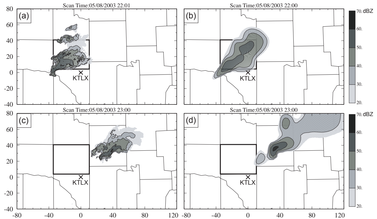
Fig. 4. Observed reflectivity fields at the 1.45^\circ elevation of the KTLX radar (left column), and the corresponding predicted reflectivity from the experiment 10B30E30LH (right column), at 2200 and 2300, 8 May 2003. The reflectivity contours are at 30, 40, 50, and 60 dBZ. The domain shown is the same as Fig. 3.
