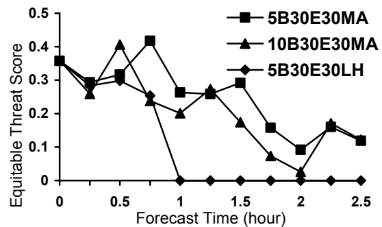
Fig. 9. Equitable threat scores of predicted reflectivity for the 45 dBZ threshold for experiments 5B30E30MA, 5B30E30LH, and 10B30E30MA.
