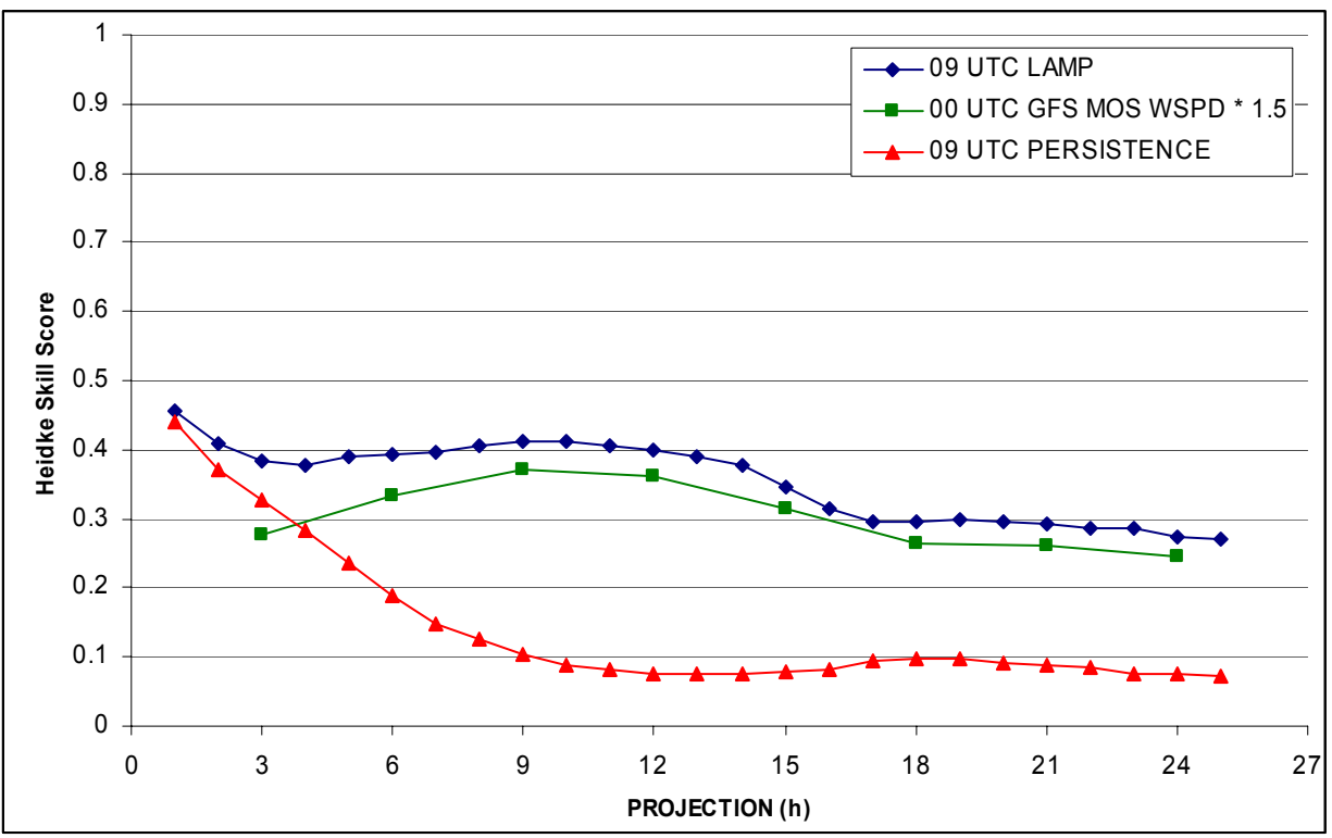
Figure 6. Heidke Skill Score for Wind Gusts for the 2004 Warm Season
