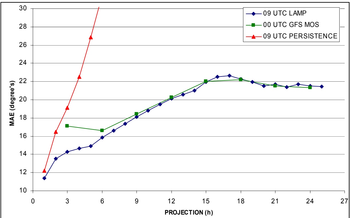
Figure 2. MAE Score for the 2004 Warm Season Wind Direction
