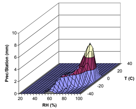
Fig. 3 Regional Dependence of Precipitation
