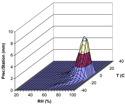
Fig. 2 Seasonal Dependence of Precipitation
