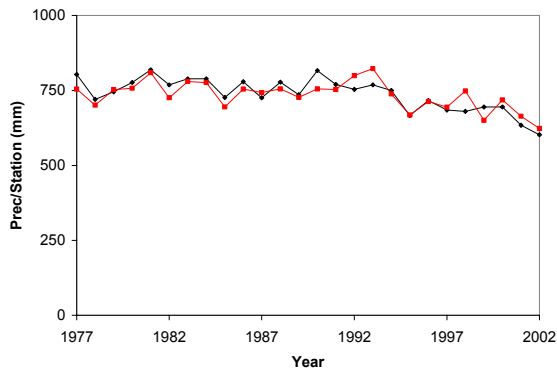
Fig. 4 Validation of Precipitation Estimation Algorithm. The black (red) curve is the observed (estimated) precipitation.
